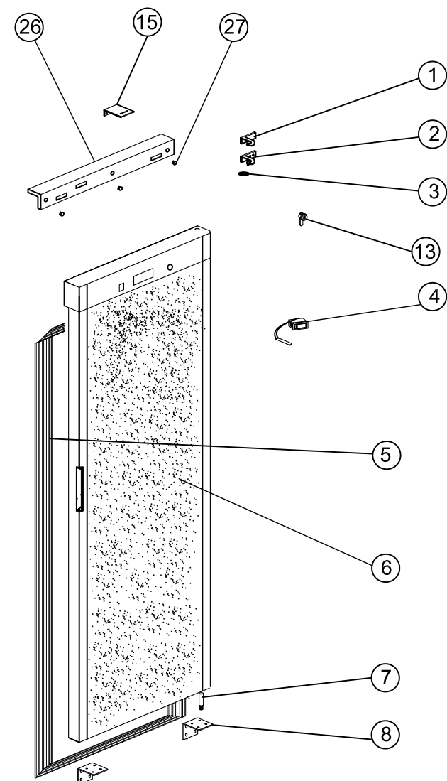
EXPLODE OF G-HT600FG
