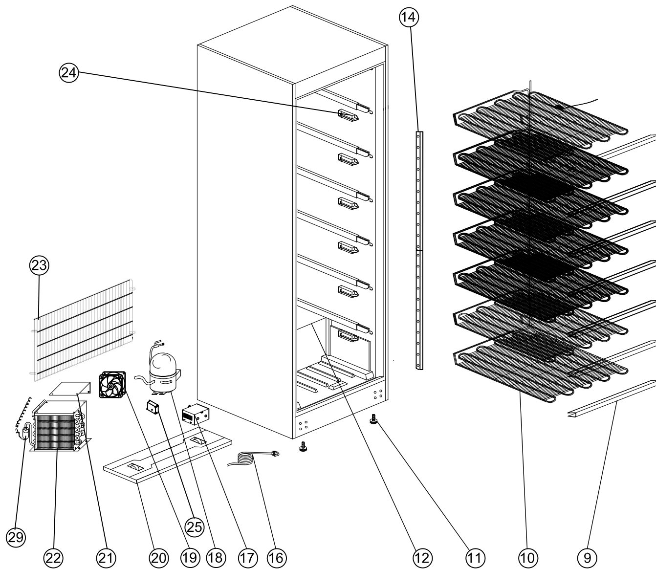
EXPLODE OF G-HT600FG
