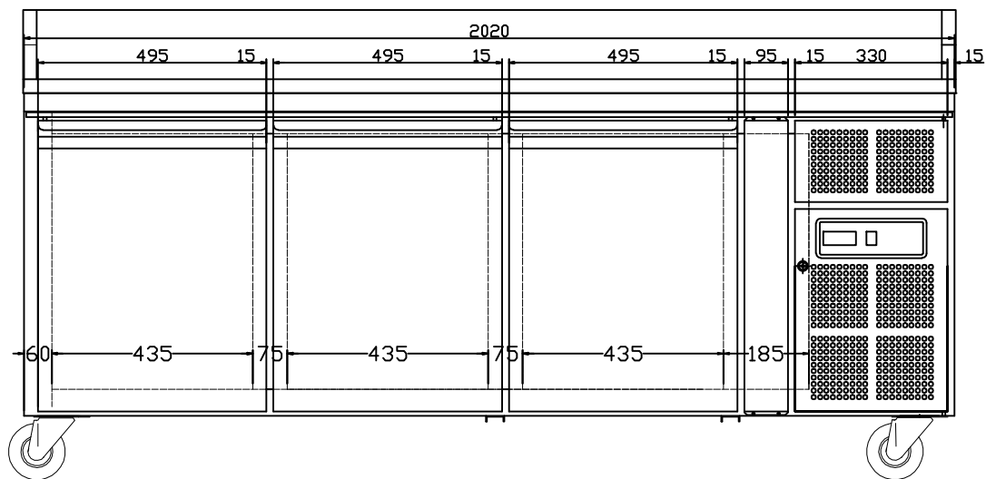
OUTSIDE SIZE OF PZ3600TN
